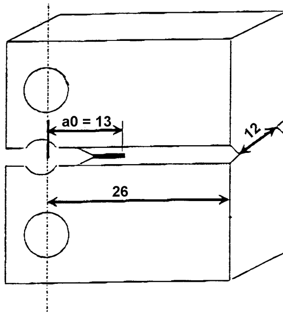
Fig. 4 CT specimen shape used (side notches)
