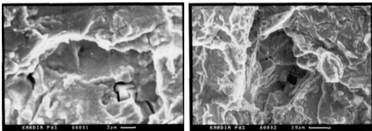
Fig. 7 Transgranular surface at the fracture of specimen PC-3
