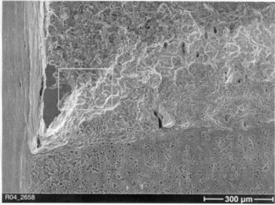
Fig. 8 Creep-related crack extension on specimen E 63.23
