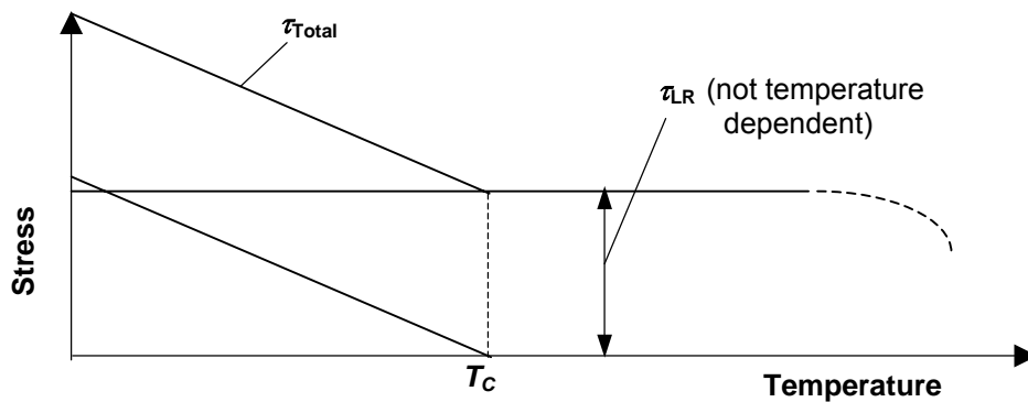
Fig. 2 Representation of the Arrhenius equation (EQ. 2) in a graph
