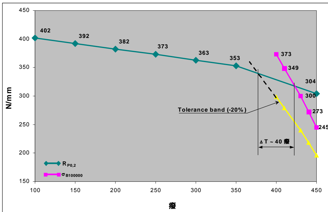
Fig. 3 Yield points and long-term strength ranges / establishment of the cut-off point
