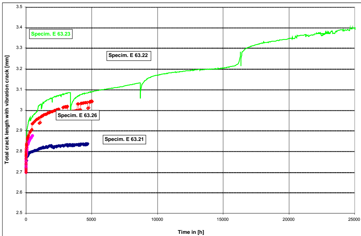
Fig. 5 Total crack lengths as a function of time
