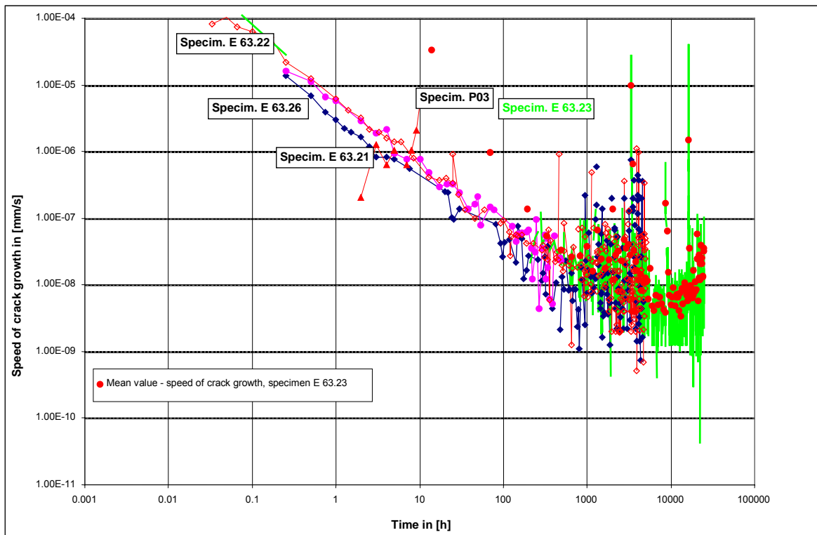
Fig. 6 Speed of crack growth as a function of time
