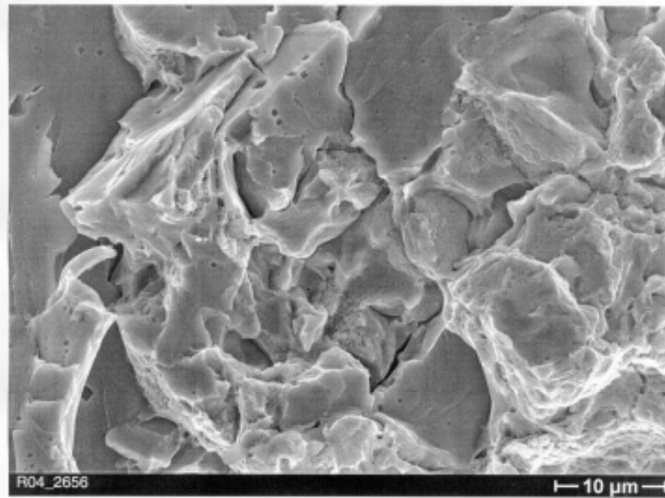
Fig. 10 Detailed record of intergranular separations from Figure 9
