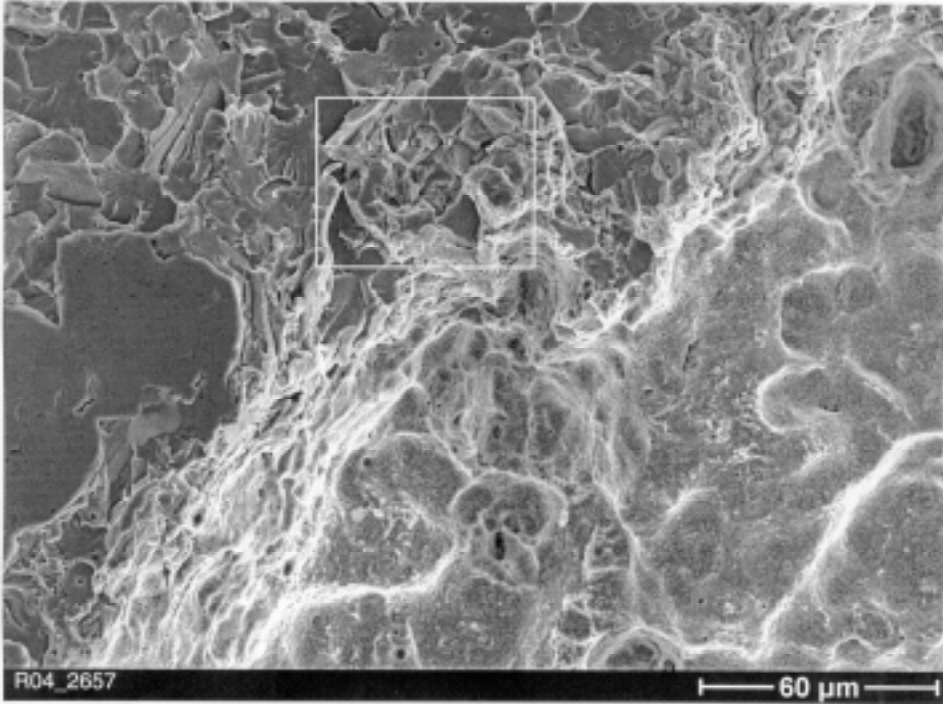
Fig. 9 Intergranular separations before the crack front, sample E 63.23 from Figure 8
